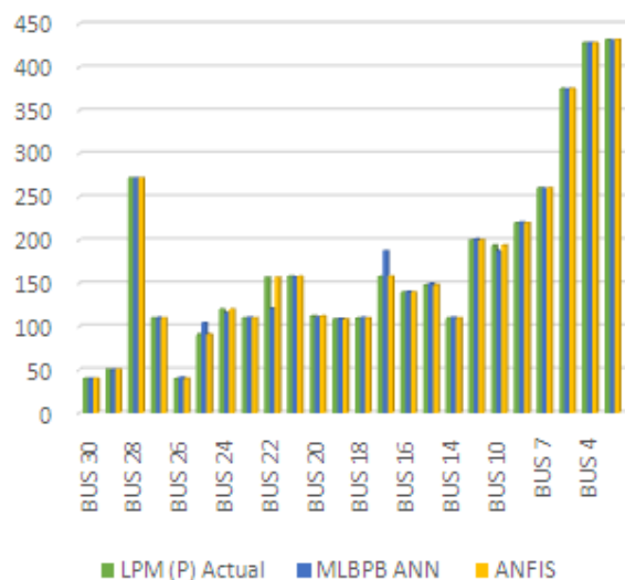
Figure-12. Comparison between the actual, MLPBP ANN and ANFIS predicted values of LPM (P).
