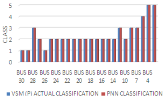
Figure-14. Comparison between the actual and PNN classification of VSM (P).
