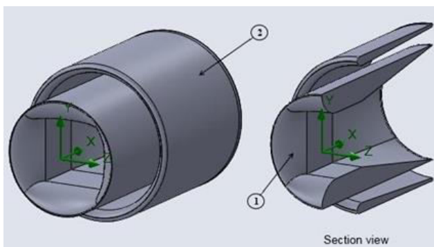
Figure-11. Main nozzle (1) with secondary diffuser (2) [2].
