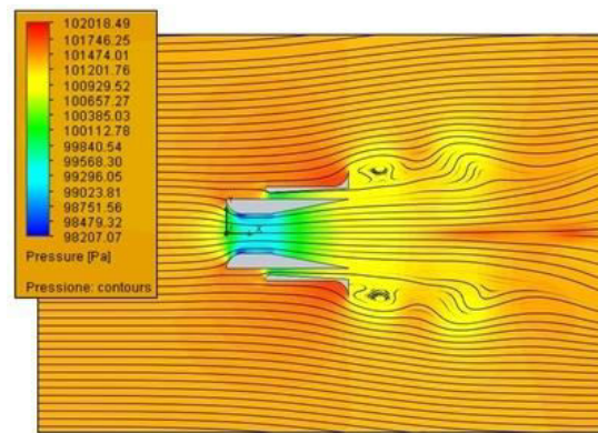
Figure-10. Effect of the secondary diffuser with a flange on the exiting flow of the divergent [2].
