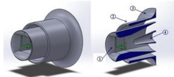
Figure-12. Section view of the final configuration. (1) Main Venturinozzle - (2) Secondary diffuser R - (3) Flange S - (4) Internal diffuser DDi.
