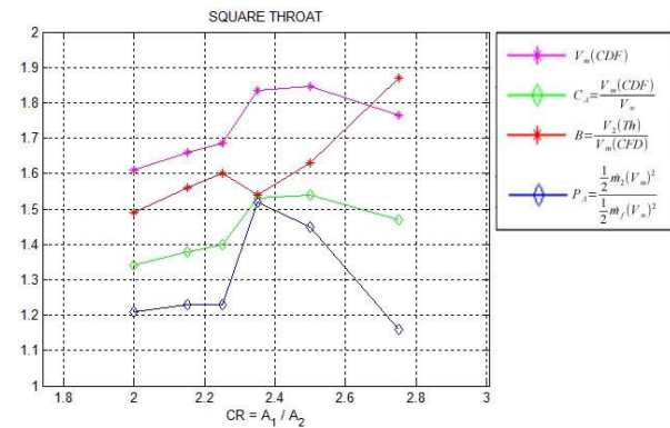
Graph-2. Trend of parameters (square throat).
