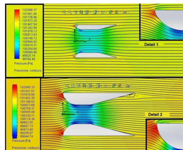
Figure-7. Streamlines and pressure trends for contraction CR=2 and CR=5 [2].
