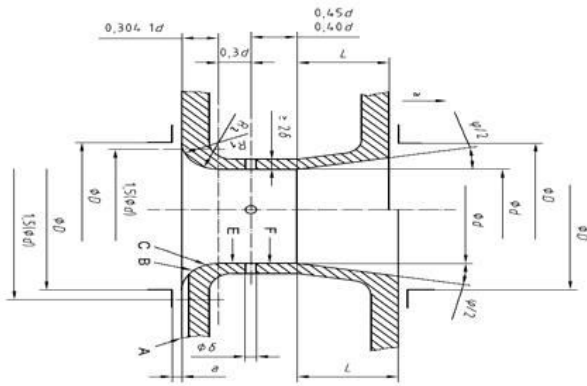
Figure-4. Venturi nozzle geometry according to ISO 5167-3 [4].
