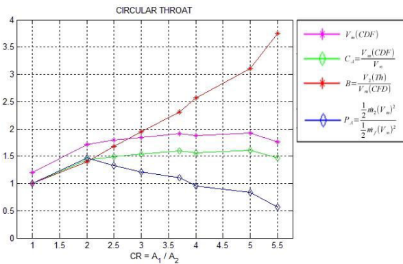
Graph-1. Trend of parameters (circular throat).
