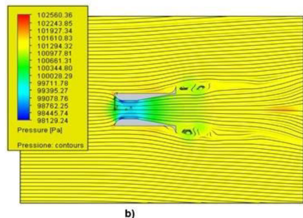
Figure-9. Flow behavior exiting the divergent without flange (a) and with flange S (b) [2].
