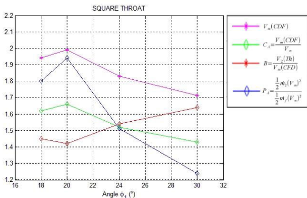
Graph-3. Trend of parameters with respect to divergent angle \phi_1 .
