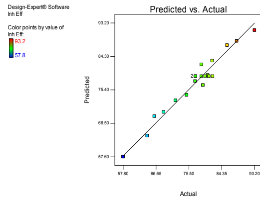
Figure-1. Plot of the predicted and actual experimental values of inhibition efficiency.
