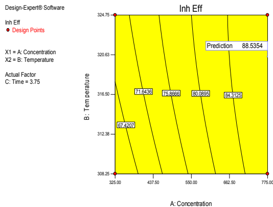
Figure-4. Effect of inhibitor concentration and temperature on inhibition efficiency.
