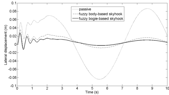
Figure-5. Lateral displacement response for 1 rad/sec excitation frequency.
