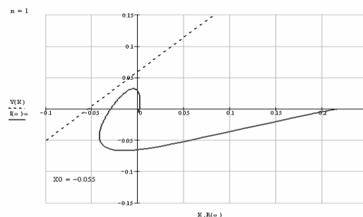
Figure-4. Relative position of the hodograph and Popov straight line n = 1 .
