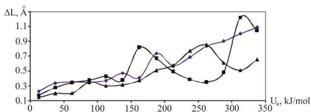
Figure-3. Changes of average values of the interlayer distance increase in the ranges of the energy of conformational rearrangements activation, 25 kJ/mol, at different degrees of coal metamorphism: 87.7% (-♦-), 89.1% (-■-), 91.26% (-▲-) [16].
