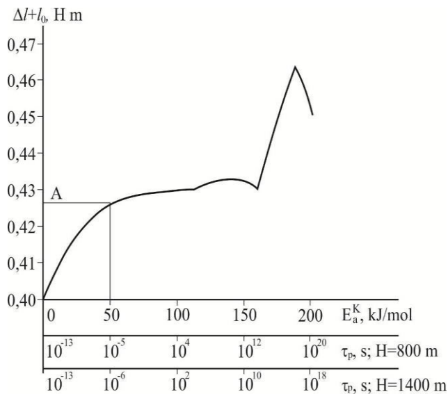
Figure-5. Dependence of the change of interlayer distances in the graphite-like layers of a coal seam on the energy of conformational rearrangements activation - E_a^k and relaxation duration - \tau_p in the molecular structure of the coal seam at its bedding depths of 800 m and 1400 m.
