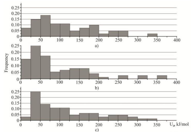
Figure-2. Histogram of frequencies of conformational rearrangement energy in the molecular structure of coal - U_a with a carbon content of 87.7% (a), 89.1% (b) and 91.26% (c) [15].
